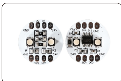
PCB board(front 2LEDs,back 2LEDs)
