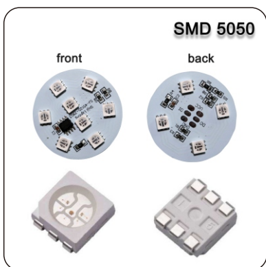
PCB board(front 8LEDs,back 4LEDs)
