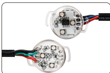
PCB board(front 3LEDs,back 3LEDs)
