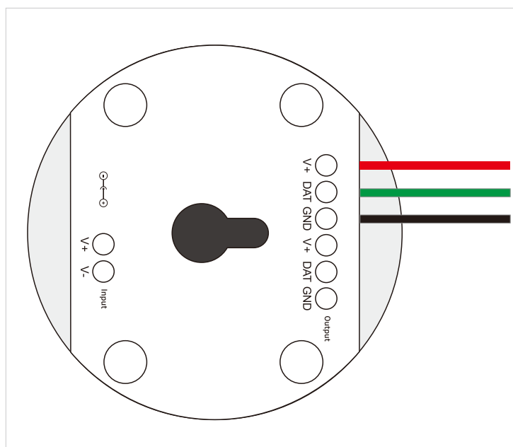
Controller and device connection
